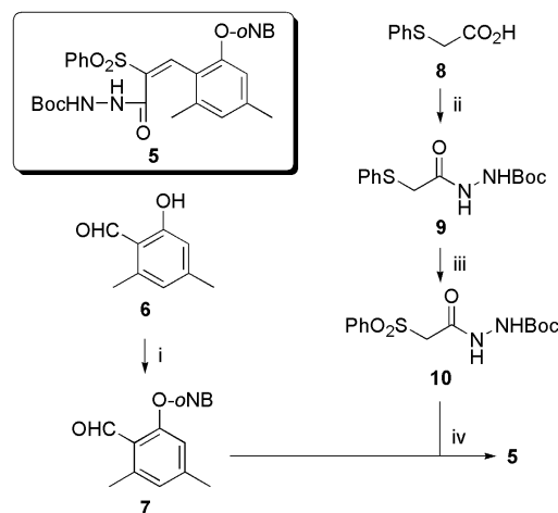
Scheme 4. Reagents and conditions: (i) o -Nitrobenzyl bromide, K_2CO_3 , CH_2Cl_2 , 77%; (ii) H_2N-NHBoc , O -(benzotriazol-1-yl)- N,N,N',N' -tetramethyluronium tetrafluoroborate (TBTU), N,N -diisopropylethylamine (DIEA), DMAP, CH_2Cl_2 , 92%; (iii) Oxone ® , MeOH/ H_2O , 0 °C to room temperature, 74%; (iv) Piperidine, AcOH, toluene, reflux, 85%. ( o NB: o -nitrobenzyl)
