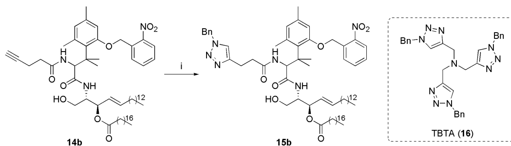
Scheme 7. Reagents and conditions. (i) benzyl azide, 0.1 eq. CuSO 4 , 0.3 eq. sodium ascorbate, 0.1 eq. TBTA ( 16 ), H 2 O/CH 2 Cl 2 = 1/1 (v/v), 91%.
