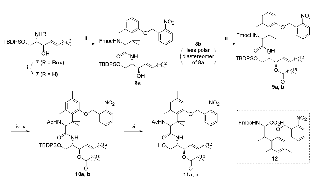
Scheme 4. Reagents and conditions. (i) TFA, \text{CH}_2\text{Cl}_2 , 76%. (ii) 12 , HBTU, N,N -diisopropylethylamine, DMF, 39% for 8a , 41% for 8b . Chemical yields of 8a derivatives are presented in following text. (iii) stearic acid, N -(3-dimethylaminopropyl)- N' -ethylcarbodiimide hydrochloride (EDC·HCl), \text{Et}_3\text{N} , DMAP, \text{CH}_2\text{Cl}_2 , 99%. (iv) piperidine, DMF. (v) AcOH, EDC·HCl, 1-hydroxybenzotriazole hydrate (HOBt· \text{H}_2\text{O} ), \text{Et}_3\text{N} , DMF, 78% (2 steps). (vi) HF, pyridine, 73%.
