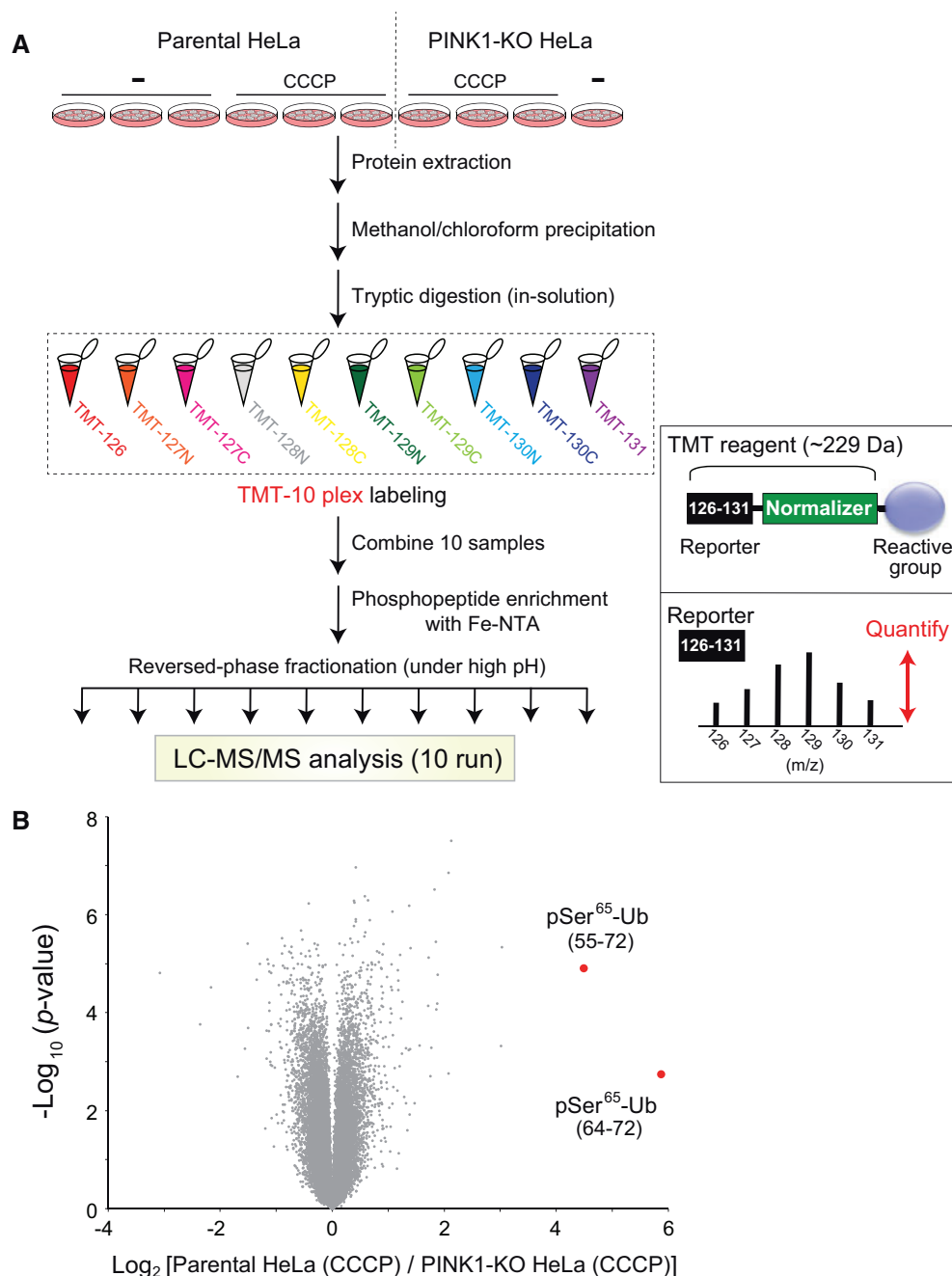
Fig. 3 Example of multiplex quantitative proteomics. (A) Workflow of the TMT/Fe(III)-nitilotriacetate (Fe-NTA)-based quantitative phosphoproteomic analysis. Parental or PINK-knockout HeLa cells (28) were treated with or without carbonyl cyanide m -chlorophenylhydrazone (CCCP). Cellular proteins were purified by methanol/chloroform precipitation and digested with trypsin. The digested peptides for each sample were labelled with TMT-10plex reagents, and all TMT-labelled samples were pooled and subjected to phosphopeptide enrichment using Fe-NTA complexes. After reversed-phase fractionation under high-pH conditions, each fraction was analysed by LC-MS/MS. Right bottom insert shows a schematic of the TMT reagent structure (top) with its functional regions (reporter and mass-normalizer) and peptide quantitation is accomplished by comparing the intensities of the reporter ions in the MS/MS spectra (bottom). (B) A volcano plot showing changes in the phosphopeptides of CCCP-treated parental HeLa cells and CCCP-treated PINK1-knockout HeLa cells. Plots of the two ubiquitin-derived peptides (corresponding to amino acids 55–72 and 64–72) containing phosphorylated Ser65 are shown in red.
