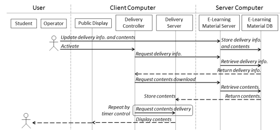
Fig. 2 System composition and processing flow of Niche-Learning
